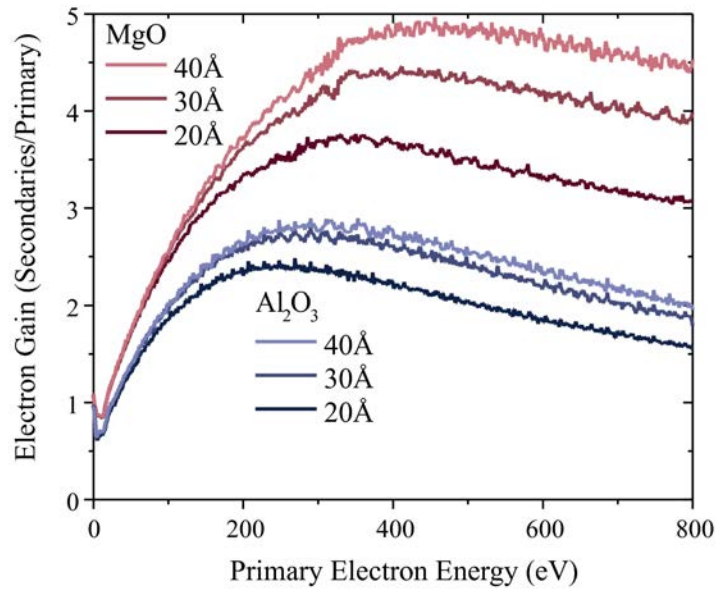
Figure 6. Measurements of the secondary emission of MgO and Al 2 O 3 versus incident electron energy [25, 26].
