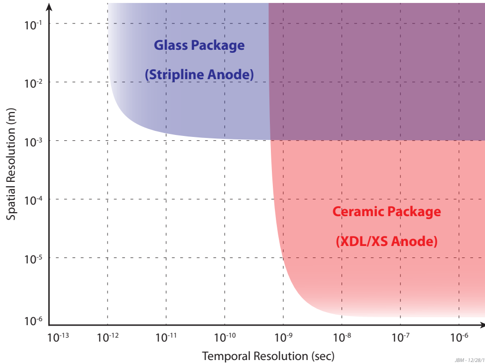
Figure 3. The contrasting performance optimizations in time and space resolution of the ceramic and glass implementations of the LAPPD™ module. The Micro-Channel Plates that form the amplification section of both detectors are identical; the difference comes from choices made for the resolution of the anode that collects the charge. The anode of the glass package consists of high bandwidth micro-strip transmission lines, optimized for time resolution [17]; the finer-detailed anode of the ceramic package has been optimized for spatial resolution [18]. (credit: J. McPhate)
