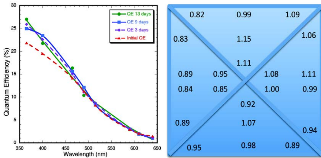
Figure 21. Left: Quantum efficiency as a function of wavelength for the 20 \times 20 \text{ cm}^2 (\text{Na}_2\text{KSb}) photocathode after transfer and sealing to the first fully-assembled LAPPD™ module while still under vacuum in the SSL tank. The tube was fully functional, with good gain and uniformity. When brought up to air one corner of the seal between the module assembly and the window leaked due to misalignment.
