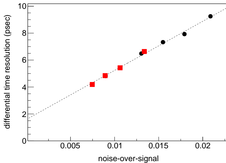
Figure 20. The time difference measured in the APS laser lab between the two ends of the module striplines versus the inverse of Signal-to-Noise in the 8" test chamber in 2012 (black circles) [3]. The error bars are smaller than the symbols. The signals are large due to the high gain; the resolution is dominated by noise from the femto-second laser. The red squares show data taken in 2014 with the Demountable chamber. The intercept of the fitted line intersects at 1.6 psec. With smaller capillary pores [46] and a signal-to-noise ratio dominated by the intrinsic noise of the PSEC4 chip we would expect sub-psec resolution [39, 3, 47].
