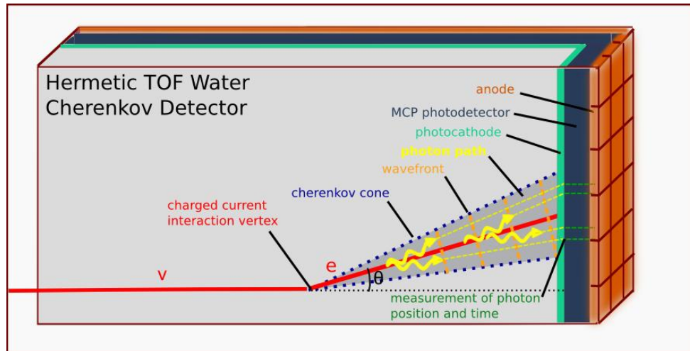
Figure 30. A 2008 conceptual drawing of a large water Cherenkov counter such as was proposed for DUSEL, in this case instrumented with LAPPDs. Note the use of time and position measurements on each Cherenkov photon to locate the track [40]. (credit: Constantinos Melachrinou)
