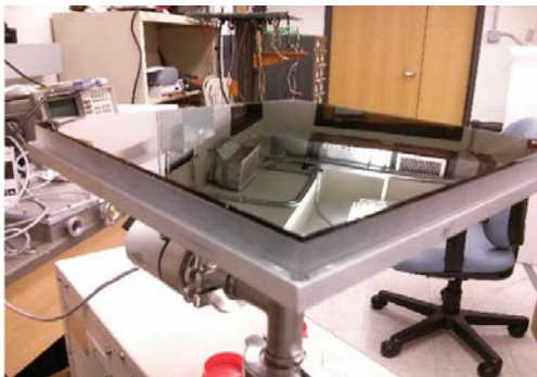
Figure 12. A glass LAPPD™ package with a hermetic indium 'flat' seal between the glass sidewall and the glass top window under test. Right: A close-up of the indium flat seal, taken through a top window with no photocathode. The photo shows the NiCr metalization on the top surface of the sidewall; a Cu layer is visible where the indium has not taken it into solution. The Cu/NiCr "finger" extending towards the bottom of the frame is for distribution of current towards the center of the cathode.
